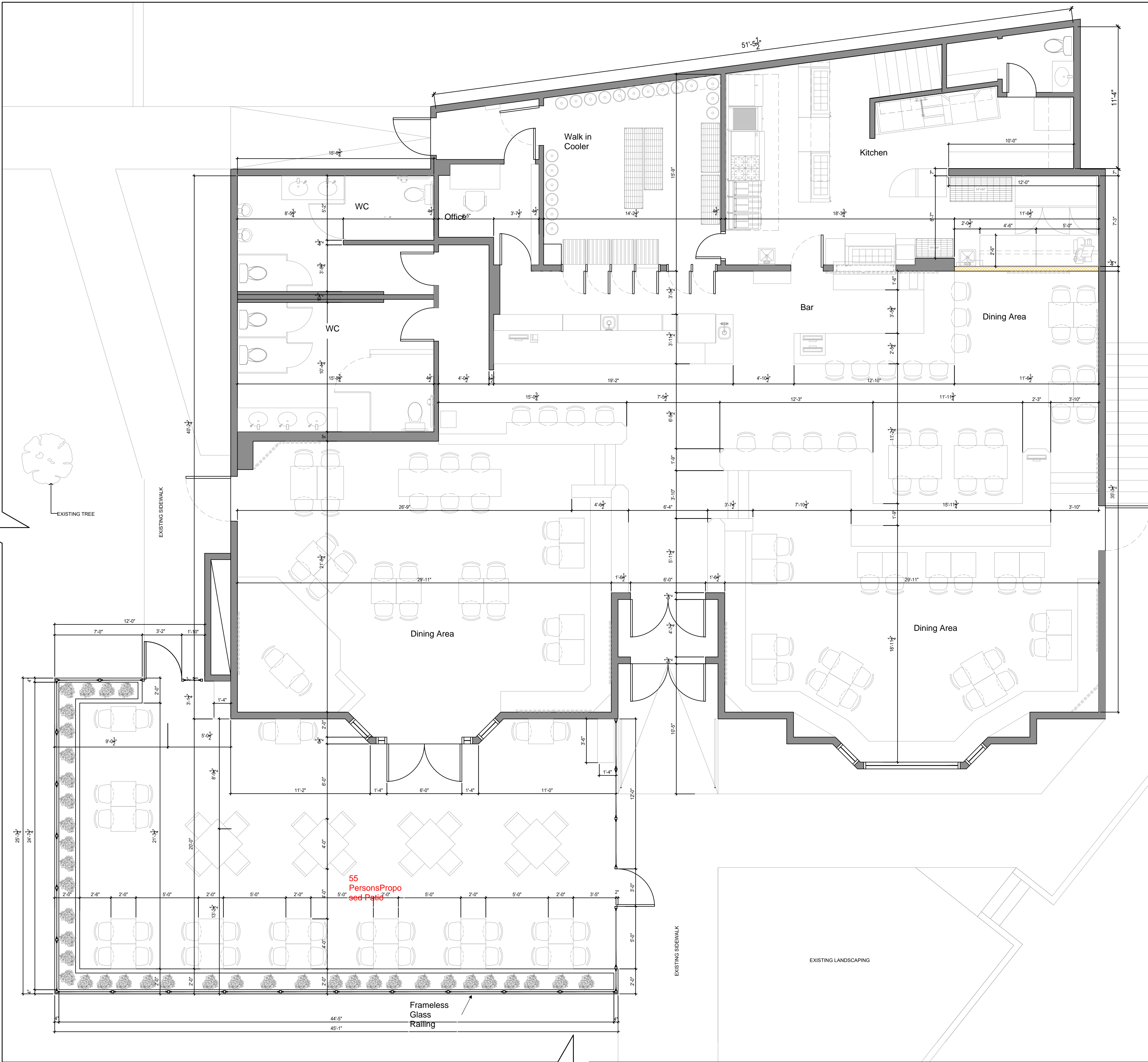
DIMENSION PLAN SCALE: 1/4" = 1'-0"
